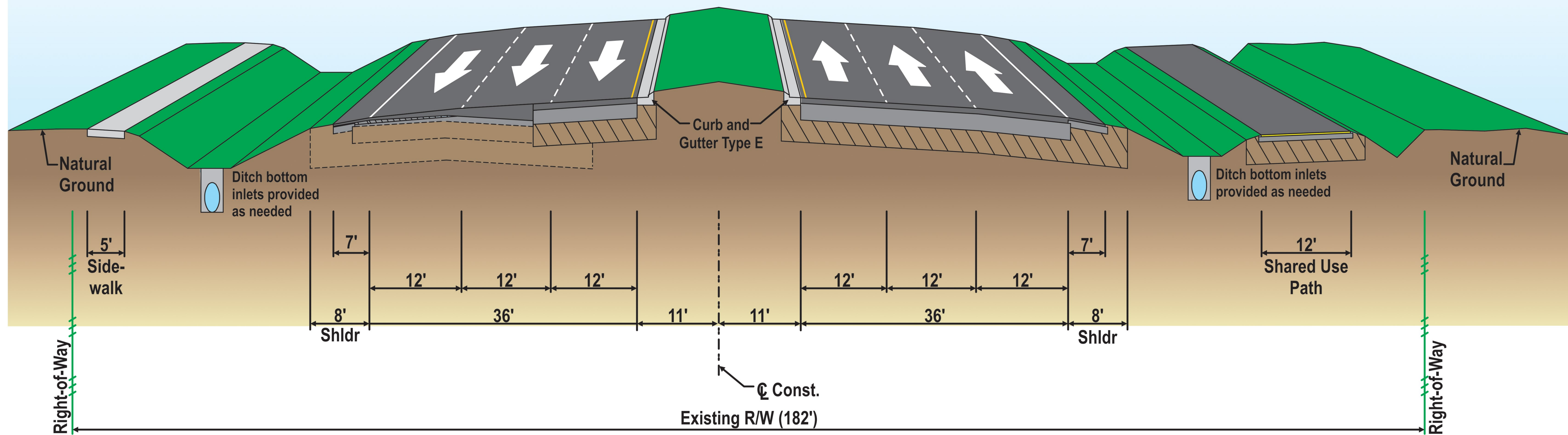
Roadway Section
