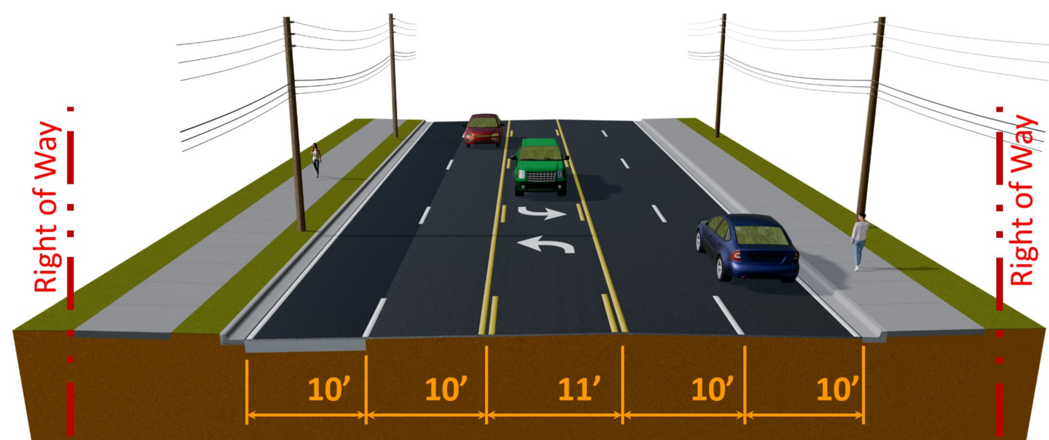
4 Lane Divided With Turn Lanes
