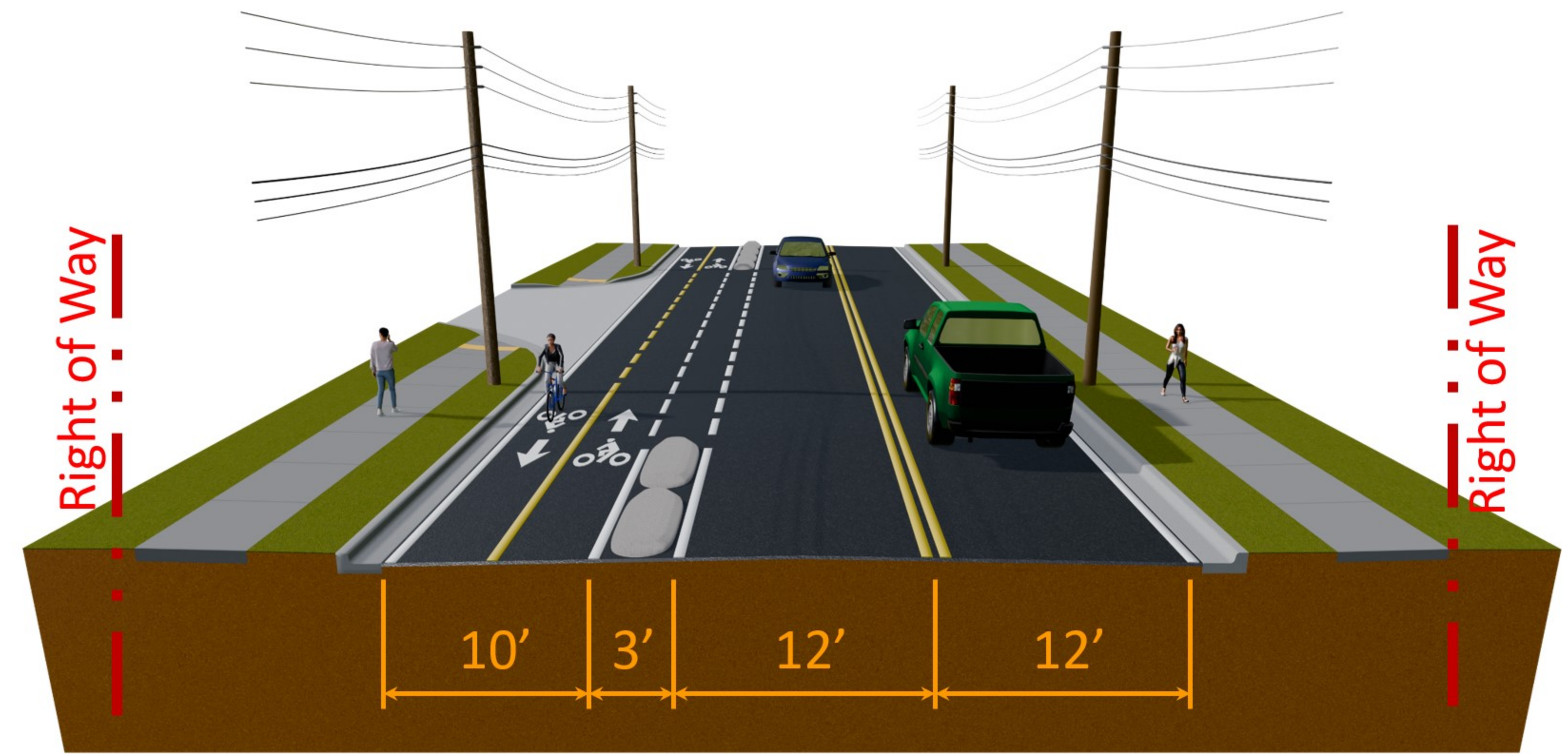
2 Lane Undivided with Protected Bicycle Facility Opportunity*
