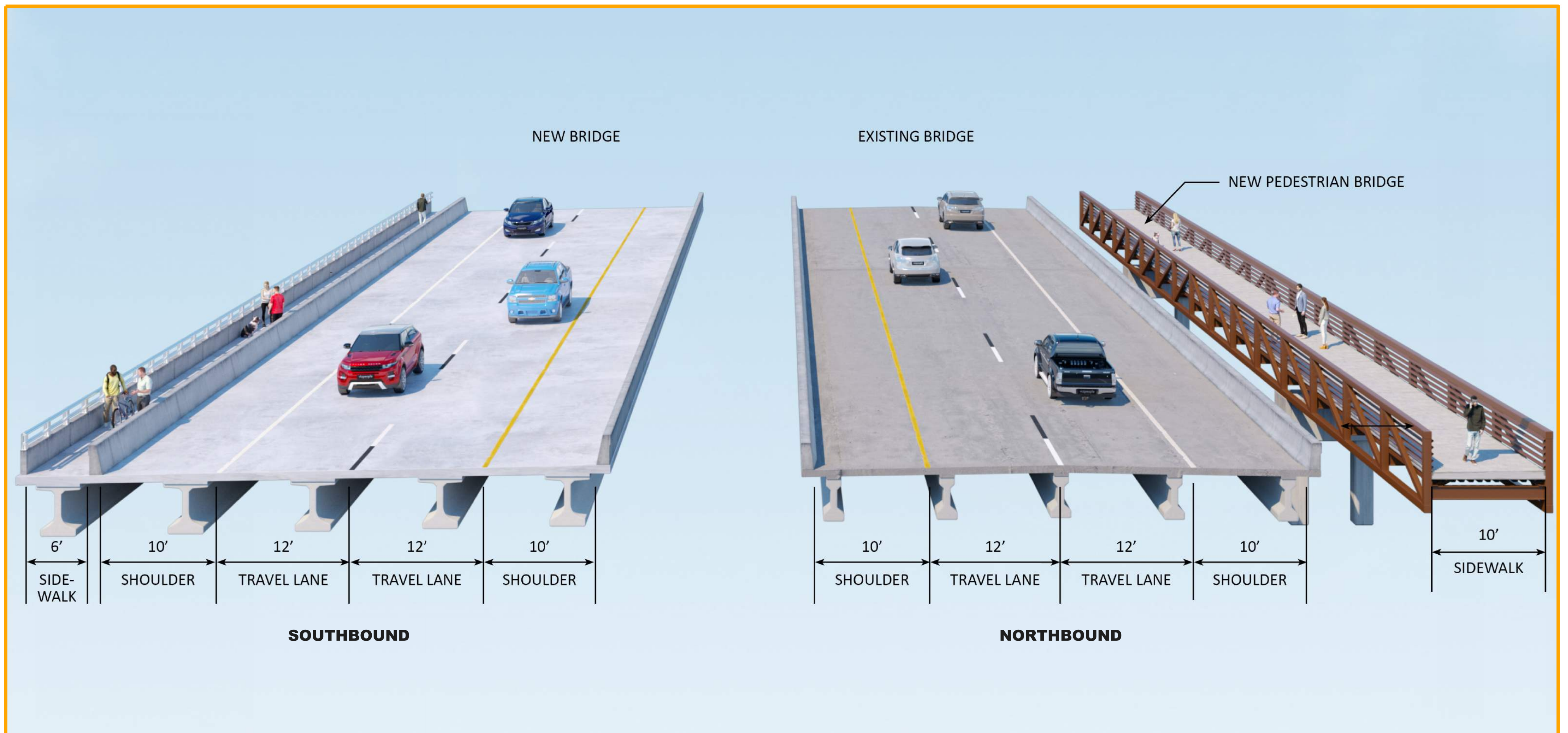
US 301 TYPICAL SECTION WITH LACOMBE RIVER BRIDGE
