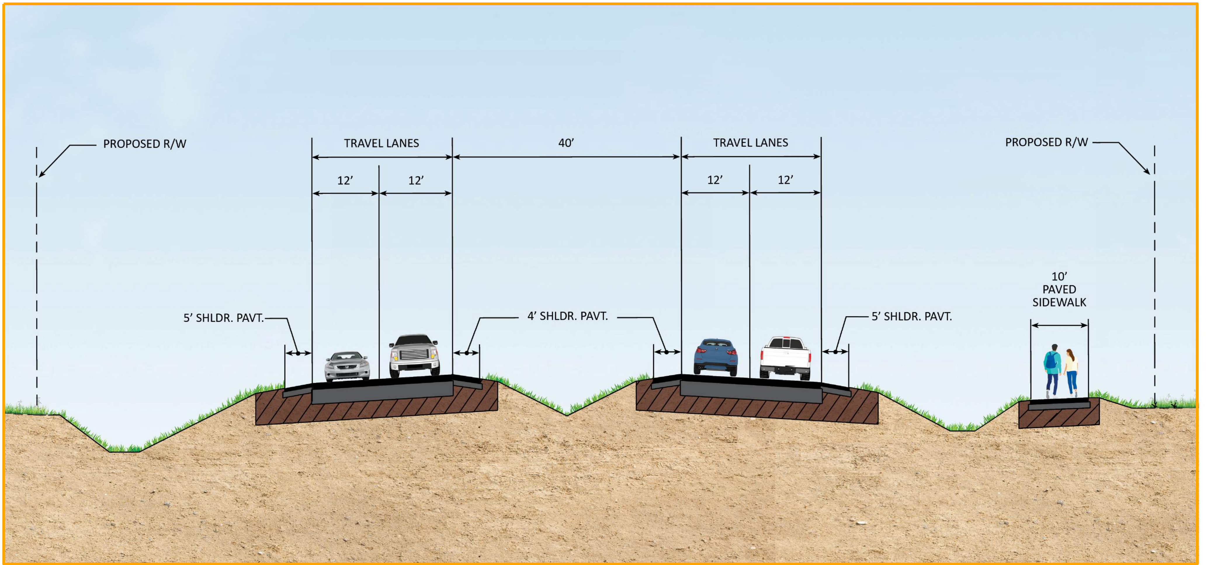
US 301 TYPICAL SECTION FROM US 98 TO SR 50/CORTEZ BLVD
